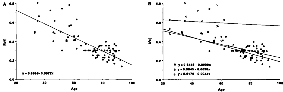
Figure 3. A: Correlation between age (years old) and |b/a| for all subjects ( r = -0.790 , p < 0.01 ). B: Correlation between age and |b/a| within the three groups. \circ (a), nAS ( r = -0.078 , p > 0.1 not sig.); \bullet (b), AS-1 ( r = -0.601 , p < 0.01 ); \blacktriangle (c), AS-2 ( r = -0.418 , p < 0.05 ).
